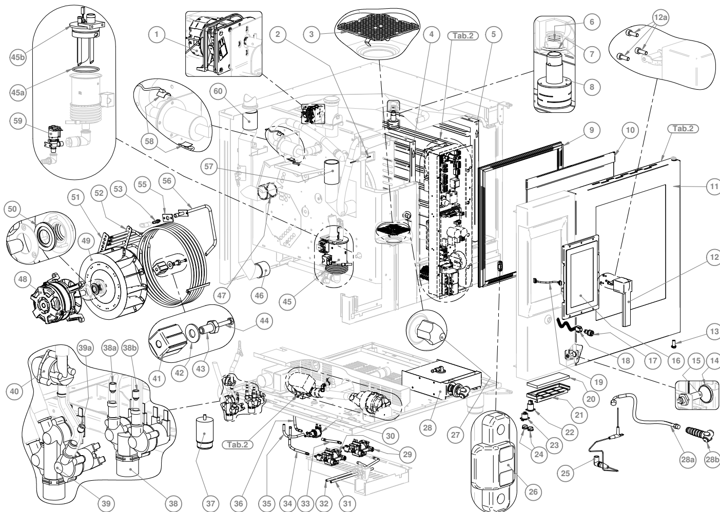
Exploded view 1/2
